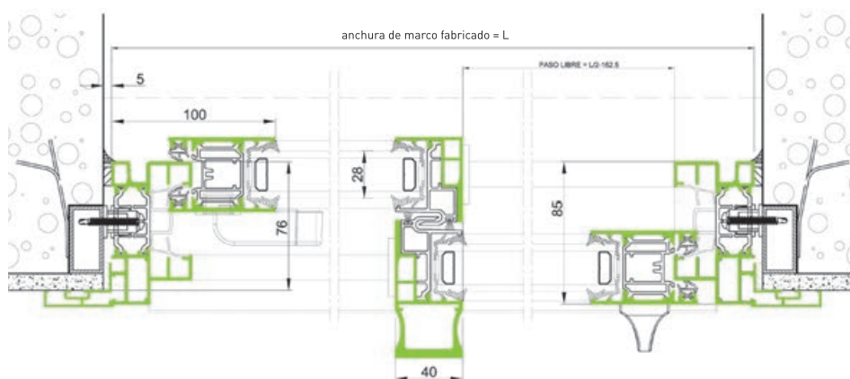
Corredera 2 railes
