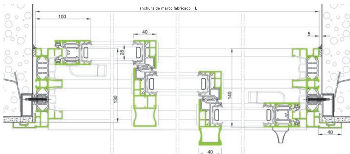
Corredera 3 railes
